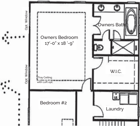
Owners Suite configuration #2 requires Opt. 4' House Depth Extension
