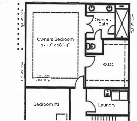
Owners Suite configuration #3 requires Opt. 4' House Depth Extension
